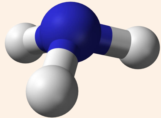
Ammonia Molecule
