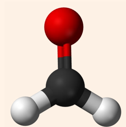
Formaldehyde Molecule
